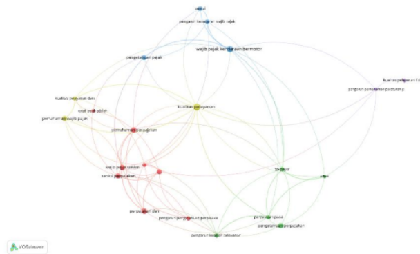
Gambar 1. Network Visualization
