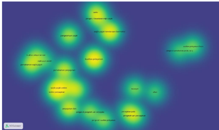
Gambar 3. Density Visualization
