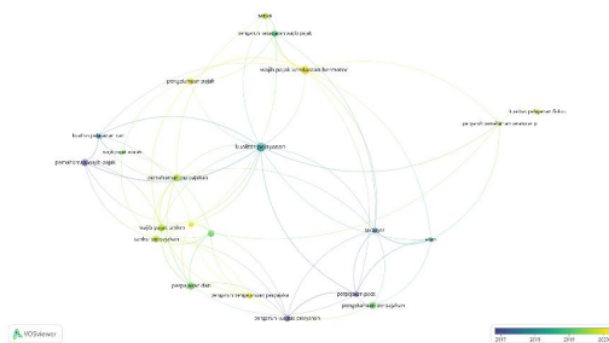
Gambar 2. Overlay Visualization
