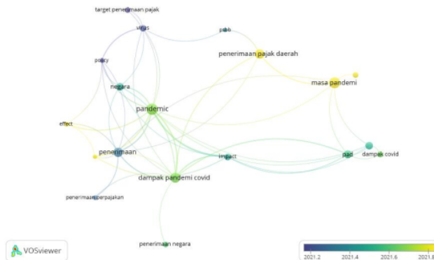
Gambar 1. Overlay Visualization
