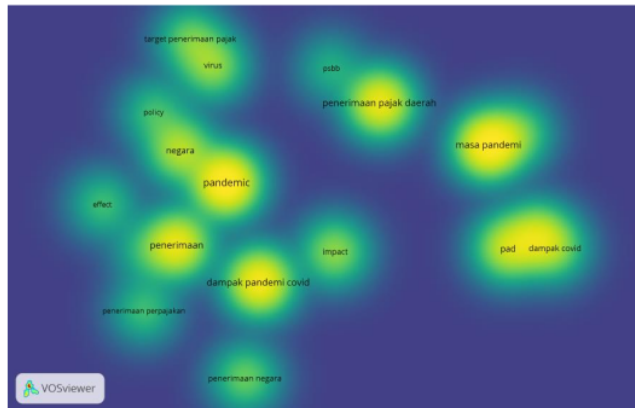
Gambar 2. Density Visualization
