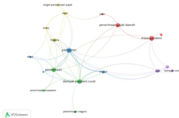
Gambar 1. Network Visualization
